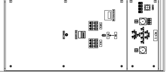
MCP-5 INNER VIEW
