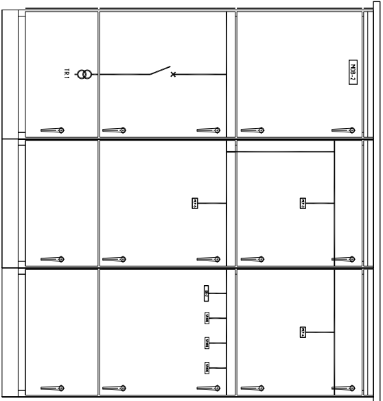
MDB2 FRONT VIEW
