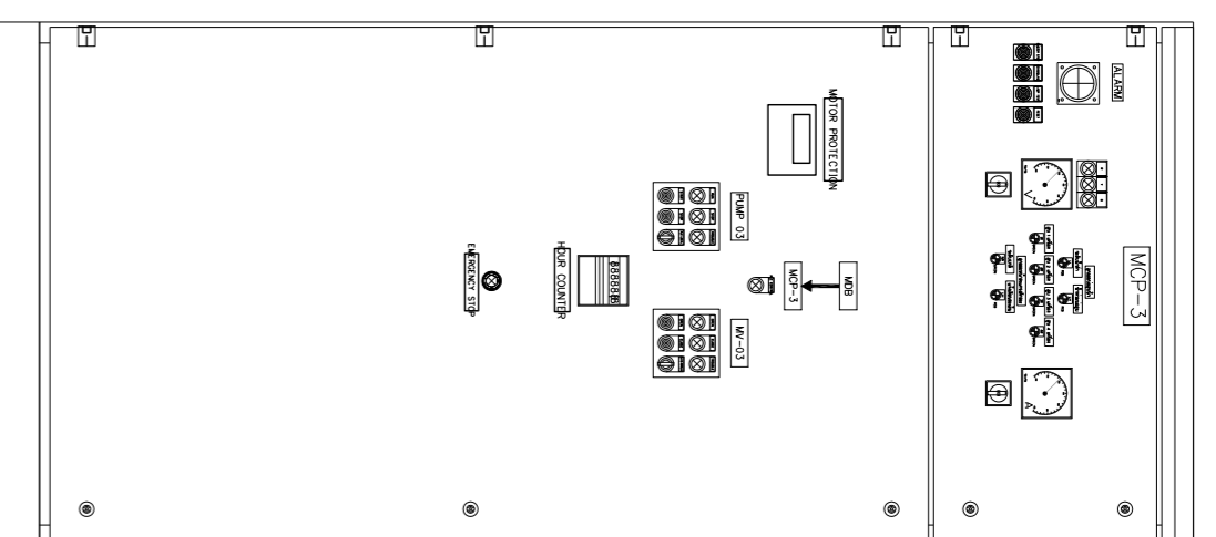
MCP-3 FRONT VIEW
